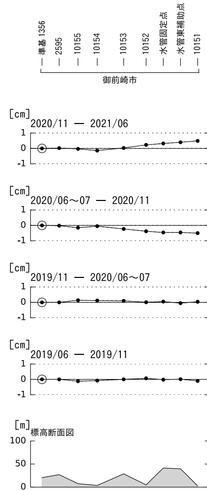
Fig. 11 Vertical crustal deformation by the precise leveling survey around Omaezaki (1/2).
