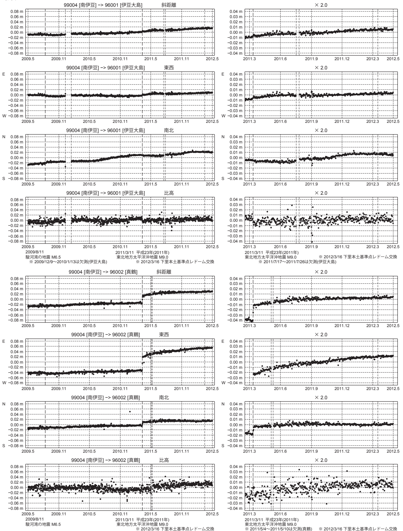
第2図 伊豆大島および真鶴のGPS連続観測結果 (2009/5/1~2012/4/30) Fig.2 Results of continuous GPS measurements for O-shima and Manazuru from May 1, 2009 to April 30, 2012.
