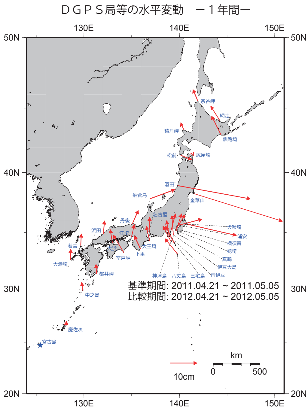
第 5 図 DGPS 局等の GPS 連続観測から求めた水平変動 Fig.5 Horizontal displacements at GPS and DGPS stations deployed by JCG, relative to Miyako Shima plotted as a solid star.
