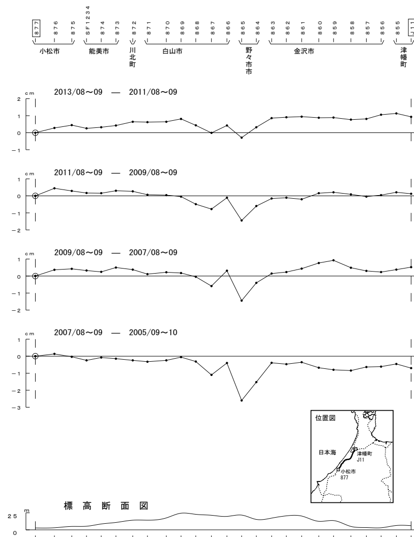
第 2 図 小松市～津幡町の上下変動 Fig. 2 Results of leveling survey along the leveling route from Komatsu city to Tsubata town.
