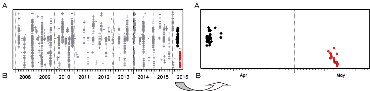
第5図(a) 三重県から奈良県の深部低周波地震活動とひずみ変化、及び推定されるゆっくりすべり領域 Fig.5(a) Activity of deep low-frequency earthquakes in Mie Prefecture to Nara Prefecture in May 2016 and strain changes, and the estimated slow slip region.
