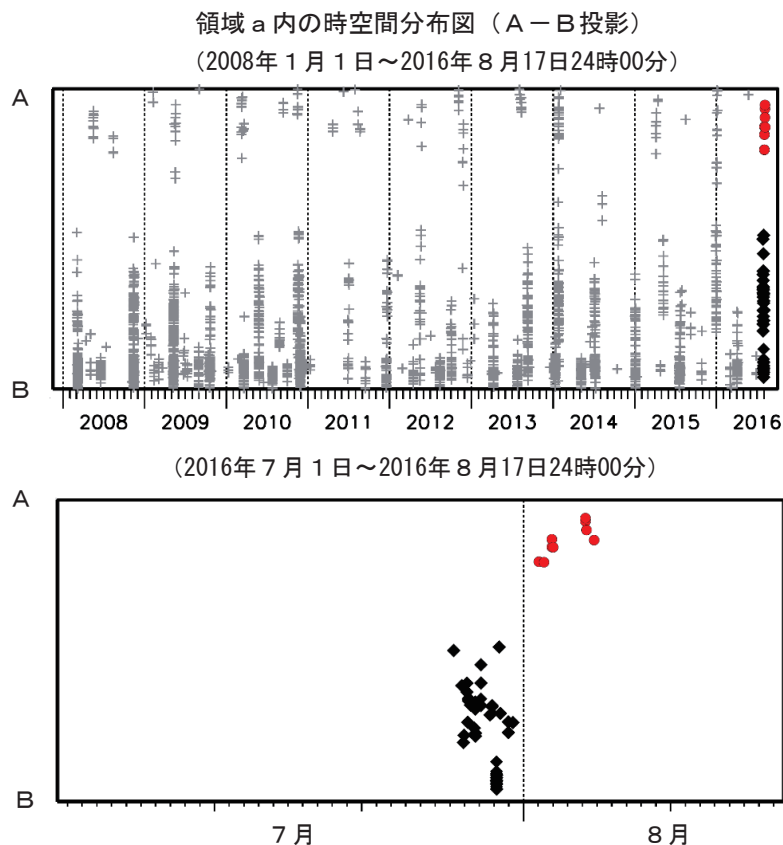
第3図(a) 三重県から愛知県の深部低周波地震活動とひずみ変化、及び推定されるゆっくりすべり領域 Fig.3(a) Activity of deep low-frequency earthquakes in Mie Prefecture to Aichi Prefecture in July - August 2016 and strain changes, and the estimated slow slip region.
