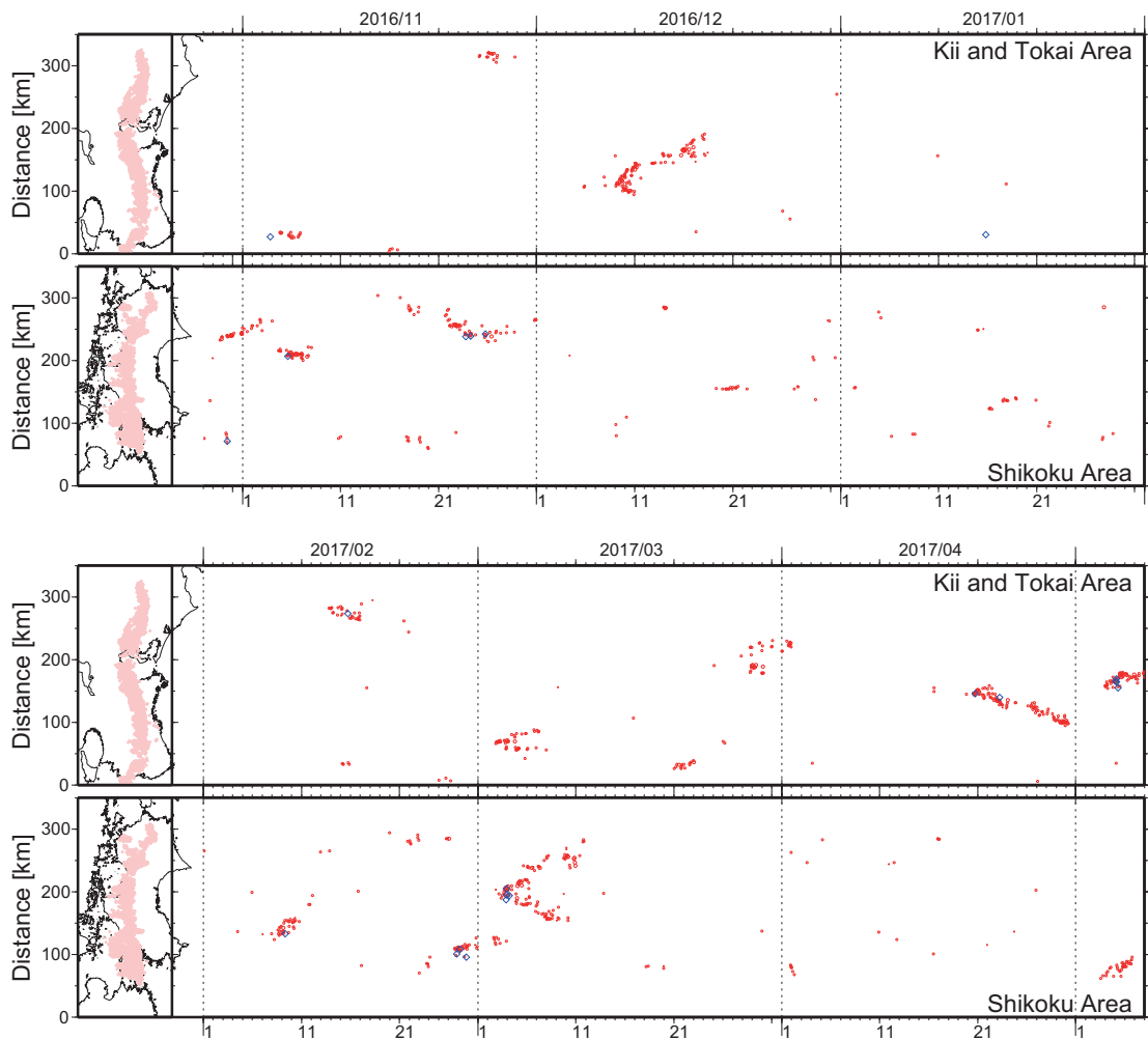
第2図 西南日本で発生した深部低周波微動（赤丸）及び深部超低周波地震（青菱形）の約6ヶ月間の時空間分布. Fig.2 Space-time plot of deep low-frequency tremor and deep very low-frequency earthquakes along the profile from southwest to northeast in southwest Japan for about six months. Red circles and blue diamonds are the same as in Fig. 1.
