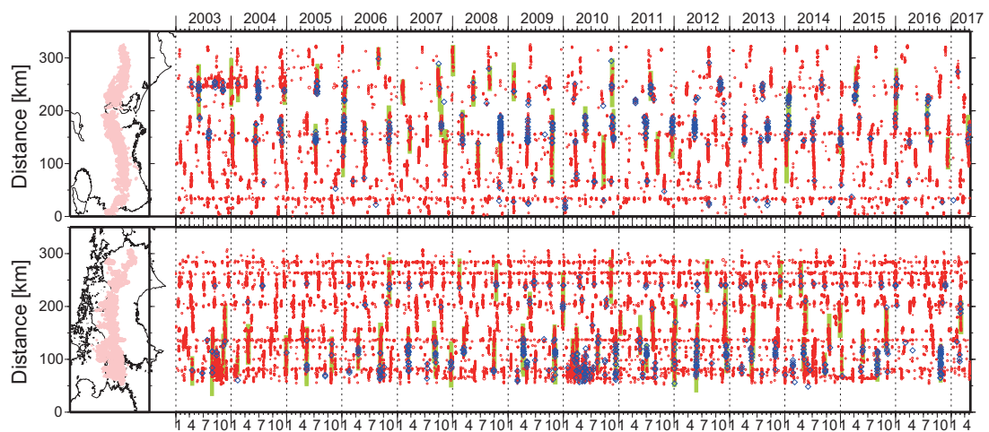
第3図 西南日本で発生した深部低周波微動（赤丸）及び深部超低周波地震（青菱形）の2003年から約14年間の時空間分布. 黄緑色太線は、傾斜変動から検出された短期的スロースリップイベントを示す. Fig.3 Space-time plot of deep low-frequency tremor and deep very low-frequency earthquakes along the profile from southwest to northeast in southwest Japan for about 14 years from January 2003. Red circles and blue diamonds are the same as in Fig. 1. Thick light green lines are short-term slow slip events detected by Hi-net tiltmeters.
