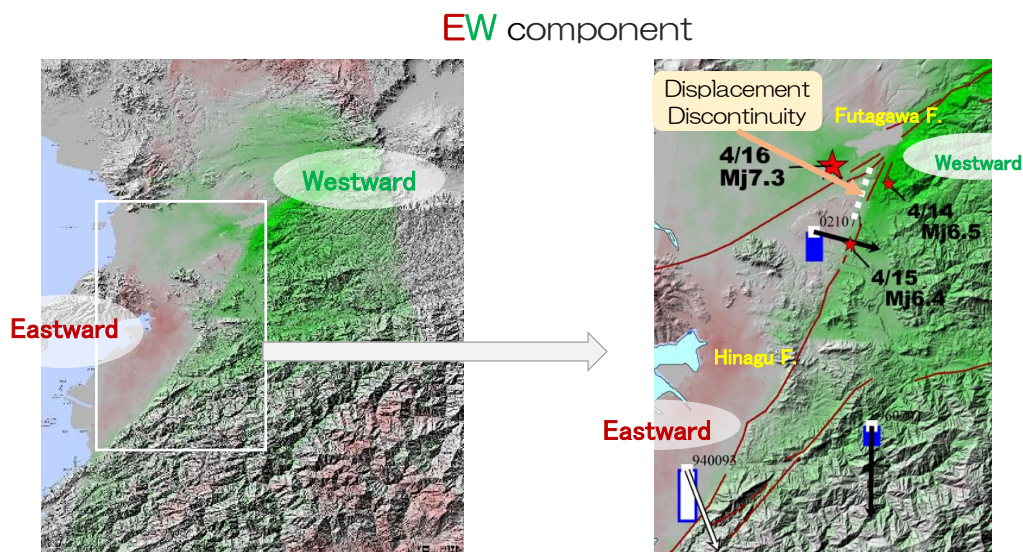
Fig. 2 InSAR-derived postseismic deformation in quasi-east-west component. Green and red represent westward and eastward displacement, respectively.
