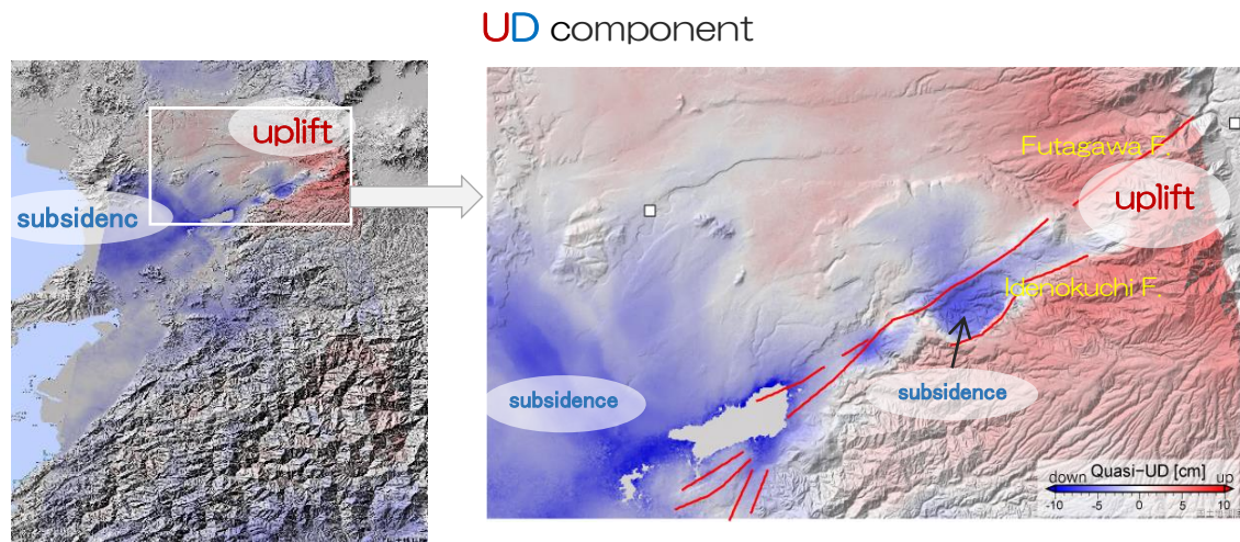
Fig. 1 InSAR-derived postseismic deformation in quasi-up-down component. Red and blue represent upheaval and subsidence, respectively.
