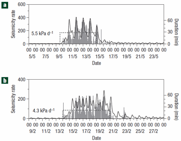
Figure 3 Comparison of calculated seismicity rate and observed tremor occurrences. a , Time series of the seismicity rate (solid line) and time sequence of the hourly tremor durations for the May 2005 swarm (bars). The left and right vertical axes indicate the seismicity rate and hourly tremor durations, respectively. The dotted box-car function indicates the extra transient stress. b , Same as a , but for the February 2006 swarm.
