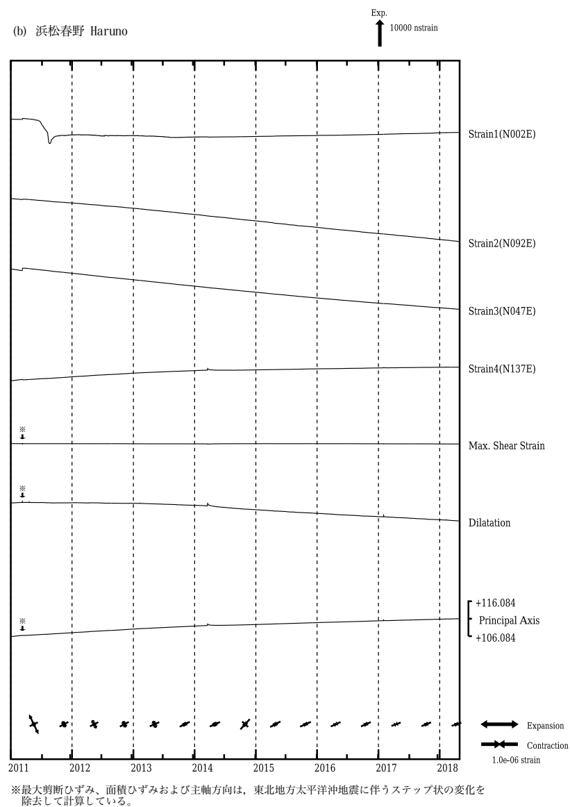
Fig. 4(a)～(e) (Left) Strain changes observed by multi-component borehole strainmeters since January 2011 (daily mean values). Principal strain, maximum shear strain and dilatation are calculated with strain values obtained from each component. (Right) Strain changes from November 2017 to April 2018 (hourly values where changes due to barometric pressure, tidal effects, geomagnetic effects and rain effects are corrected) observed by multi-component borehole strainmeters.
