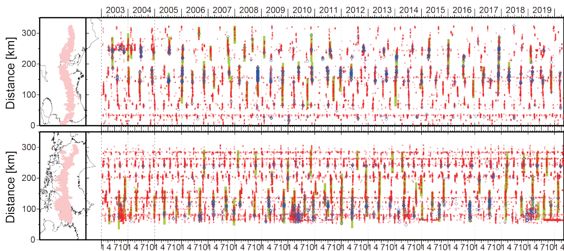
第 3 図 西南日本で発生した深部低周波微動（赤丸）及び深部超低周波地震（青菱形）の 2003 年から約 17 年間の時空間分布。黄緑色太線は、傾斜変動から検出された短期的スロースリップイベントを示す。 Fig. 3 Space-time plot of deep low-frequency tremor and deep very low-frequency earthquakes along the profile from southwest to northeast in southwest Japan for about 17 years from January 2003. Red circles and blue diamonds are the same as in Fig. 1. Thick light green lines are short-term slow slip events detected by Hi-net tiltmeters.
