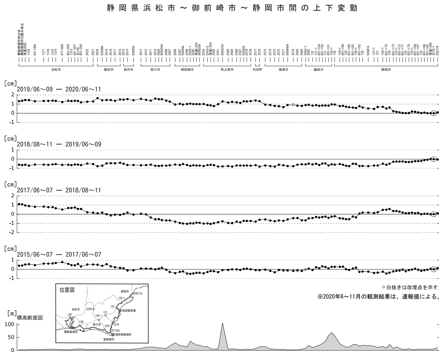
第 28 図 浜松市～御前崎市～静岡市間の上下変動 Fig. 28 Vertical displacements from Hamamatsu city to Shizuoka city via Omaezaki city.
