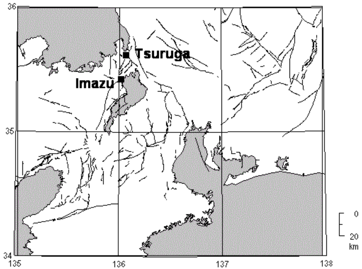
第 1 図 今津・敦賀観測点の位置. 図中の線は活断層研究会(1991) 4) による活断層の位置. Fig. 1 Locational map of crustal deformation observation stations (Imazu and Tsuruga). The lines in the figure are the position of active faults by The Research Group for Active Faults of Japan (1991).
