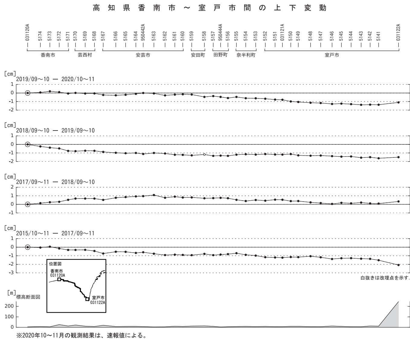
第 11 図 香南市～室戸市間の上下変動 Fig. 11 Results of leveling survey along the leveling route from Konan city to Muroto city.
