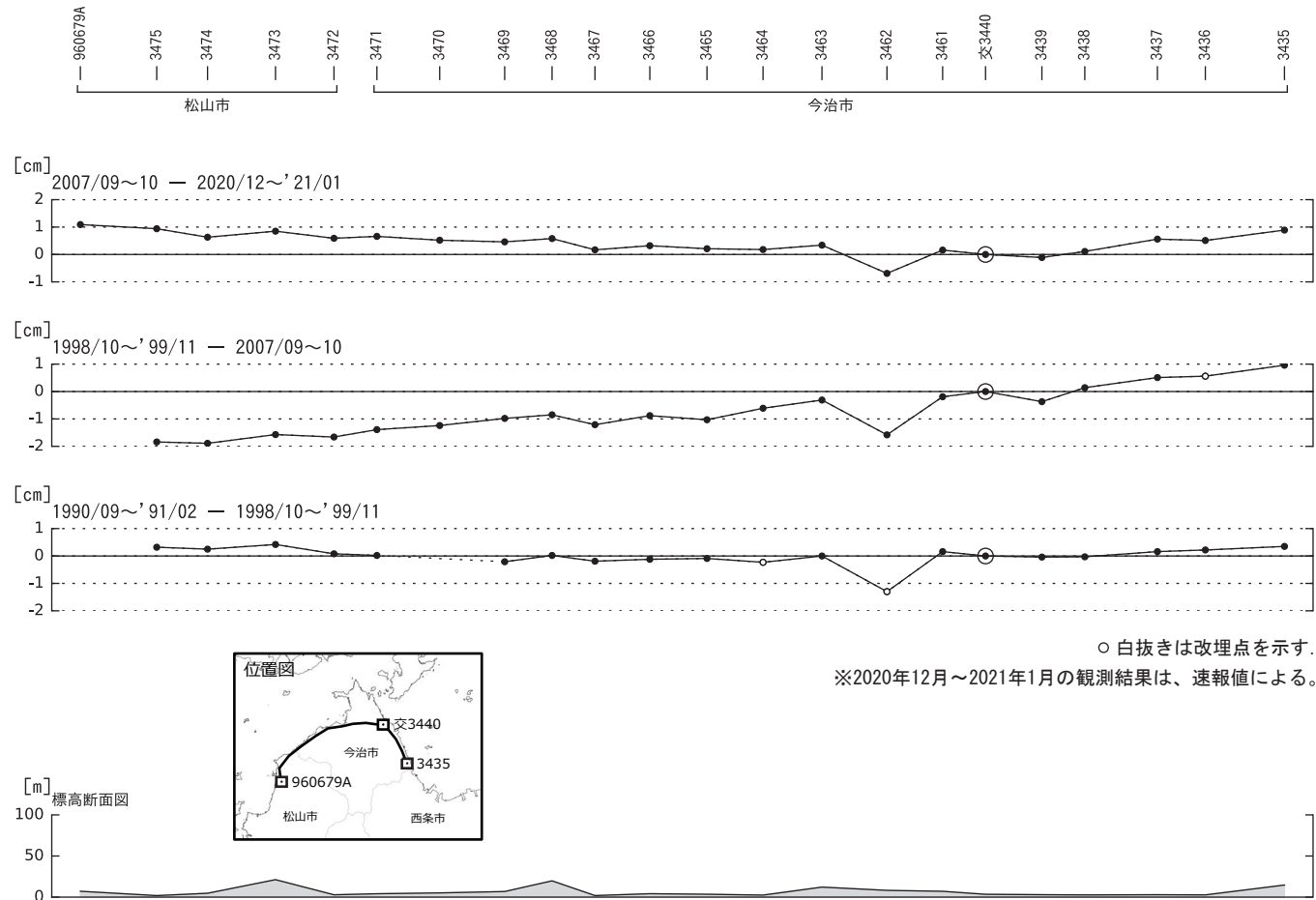
第 14 図 松山市～今治市間の上下変動 Fig. 14 Results of leveling survey along the leveling route from Matsuyama city to Imabari city.
