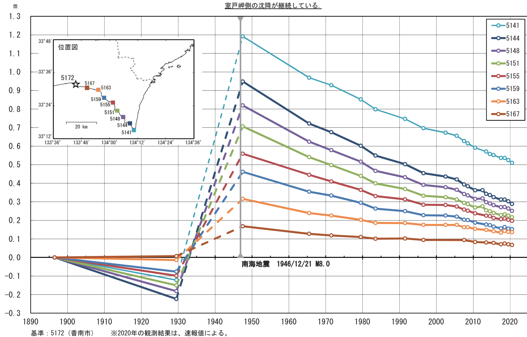
第 13 図 水準点 5172 (香南市) を基準とした室戸岬周辺の各水準点の高さの上下変動時系列 Fig. 13 Time series of height changes of benchmarks along the leveling route on the coast of the Muroto Peninsula from BM5172 (Konan) to BM5141 (Muroto) referred to BM5172 (Konan).
