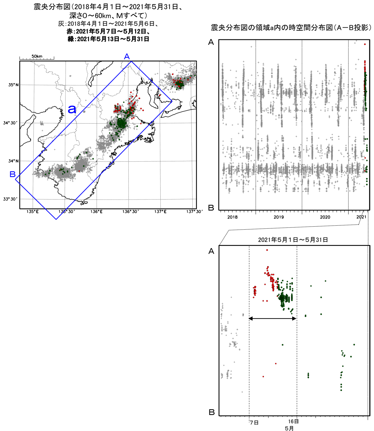
Fig. 6(a) Activity of deep low-frequency earthquakes in northern part of Kii Peninsula and strain changes, and the estimated slow slip region.
