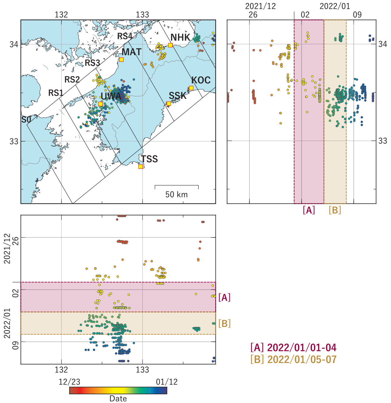
第 25 図 四国西部における低周波地震（気象庁一元化カタログによる）の時空間分布（2021/12/23 ～ 2022/01/11）. Fig. 25 Space-time distribution of low-frequency earthquakes by JMA unified hypocenter catalog in the Western Shikoku from December 23, 2021 to January 11, 2022.
