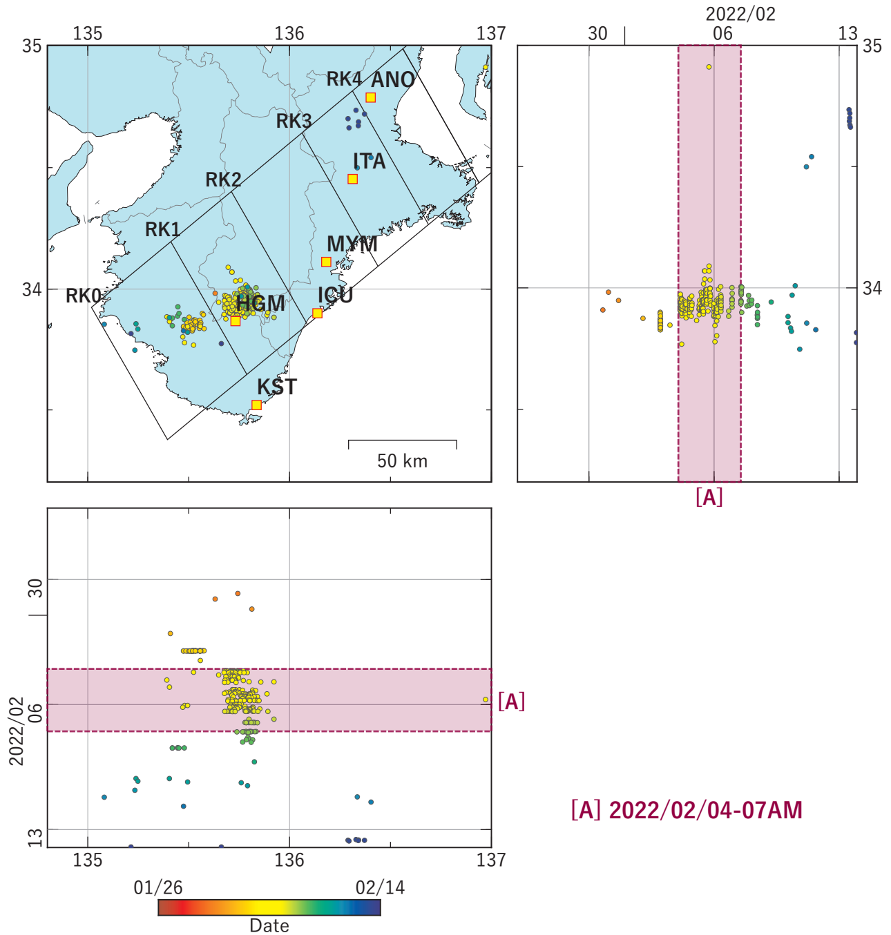
第 33 図 紀伊半島における低周波地震（気象庁一元化カタログによる）の時空間分布（2022/01/26 ～ 2022/02/13）. Fig. 33 Space-time distribution of low-frequency earthquakes by JMA unified hypocenter catalog in the Kii Peninsula from January 26 to February 13, 2022.
