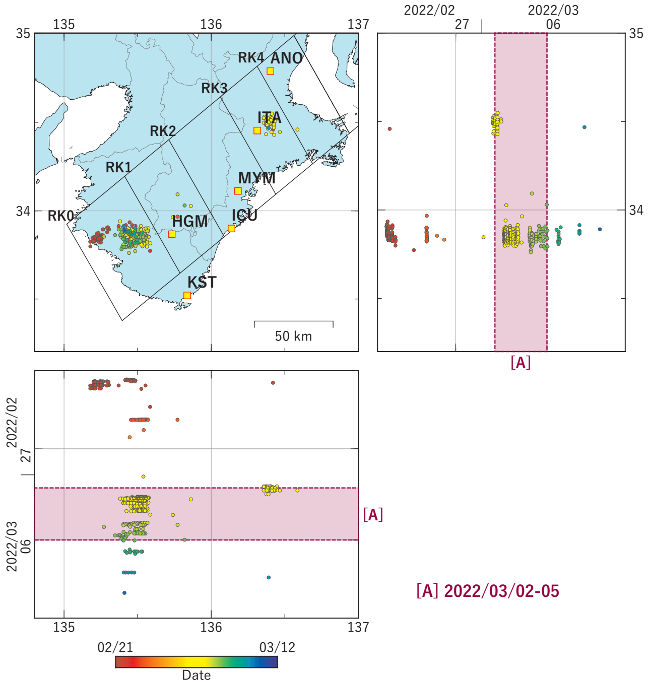
第 39 図 紀伊半島における低周波地震（気象庁一元化カタログによる）の時空間分布（2022/02/21 ～ 2022/03/11）. Fig. 39 Space-time distribution of low-frequency earthquakes by JMA unified hypocenter catalog in the Kii Peninsula from February 21 to March 11, 2022.
