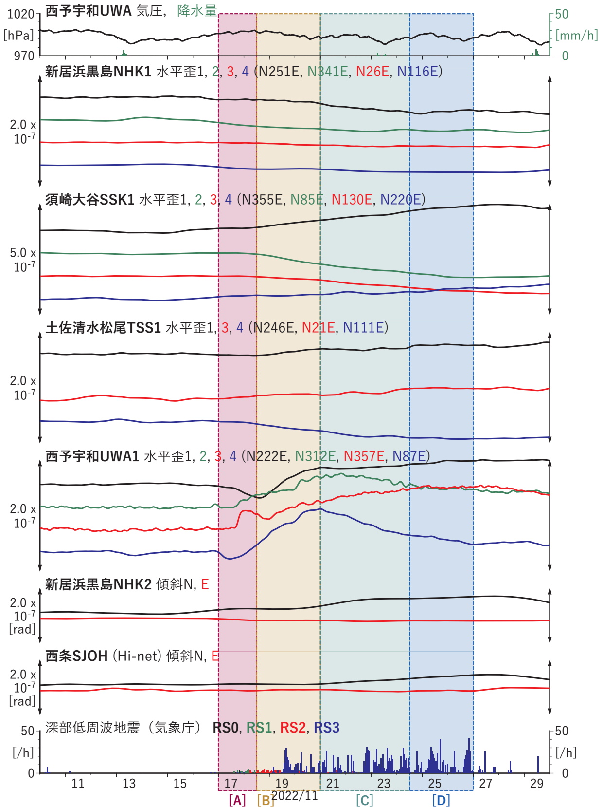
第 8 図 四国西部における歪・傾斜の観測結果と低周波地震の検出数 (2022/11/10 ~ 2022/11/29). Fig. 8 Observed strain and tilt data and detected number of low-frequency earthquakes in the Western Shikoku from November 10 to 29, 2022.
