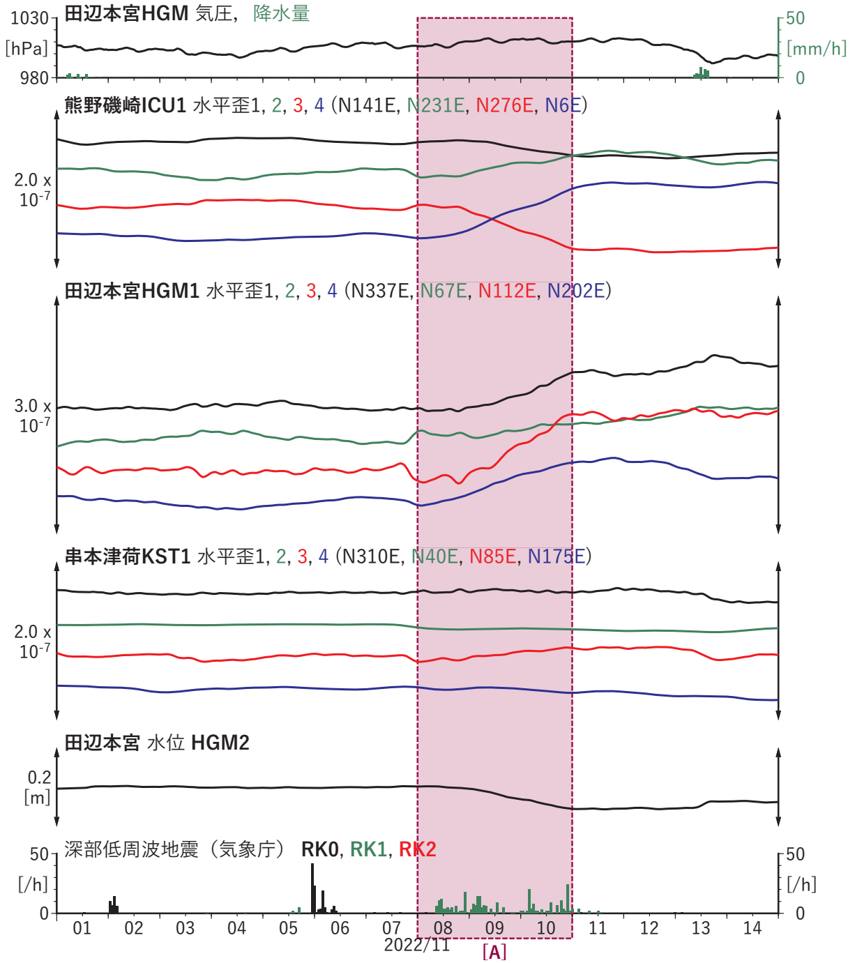
第 5 図 紀伊半島における歪・傾斜・地下水位の観測結果と低周波地震の検出数 (2022/11/01 ~ 2022/11/14). Fig. 5 Observed strain, tilt and groundwater level data and detected number of low-frequency earthquakes in the Kii Peninsula from November 01 to 14, 2022.
