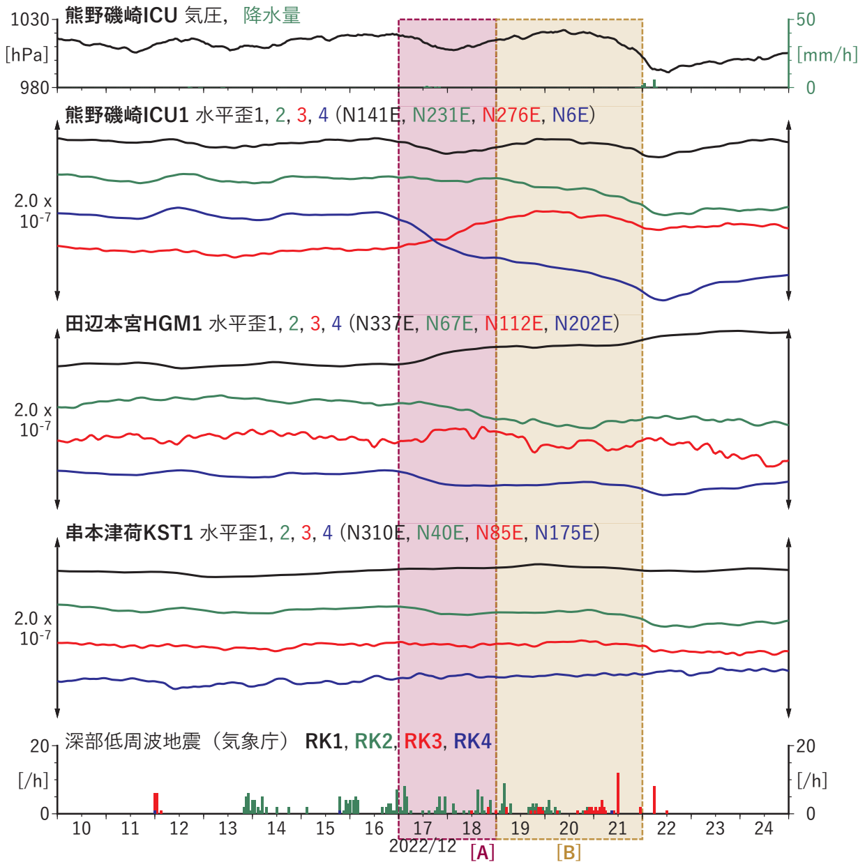
第 14 図 紀伊半島における歪・傾斜の観測結果と低周波地震の検出数 (2022/12/10 ~ 2022/12/24). Fig. 14 Observed strain and tilt data and detected number of low-frequency earthquakes in the Kii Peninsula from December 10 to 24, 2022.
