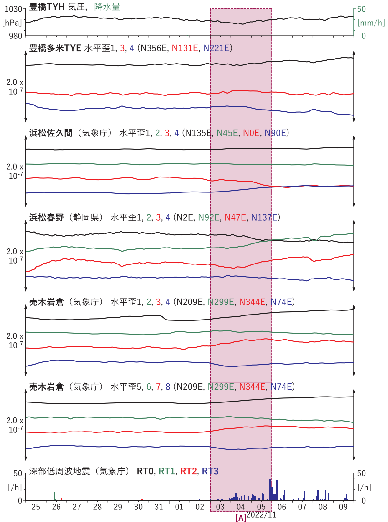
第 2 図 東海地域における歪・傾斜の観測結果と低周波地震の検出数 (2022/10/25 ~ 2022/11/09). Fig. 2 Observed strain and tilt data and detected number of low-frequency earthquakes in the Tokai region from October 25 to November 09, 2022.
