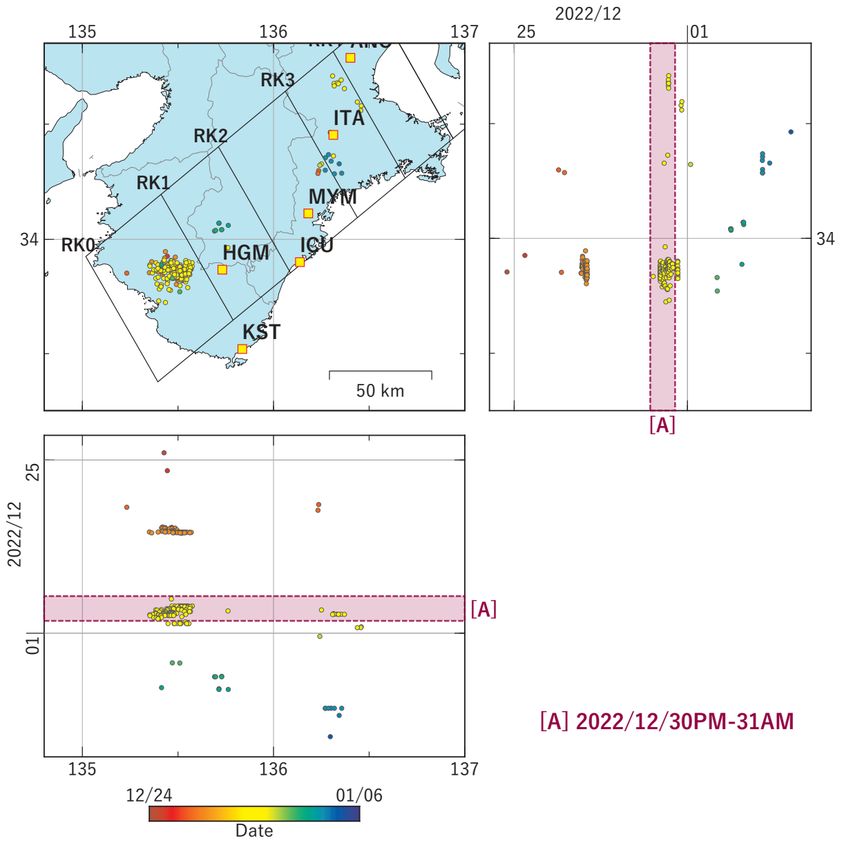
第 17 図 紀伊半島における低周波地震（気象庁一元化カタログによる）の時空間分布（2022/12/24 ～ 2023/01/05）. Fig. 17 Space-time distribution of low-frequency earthquakes by JMA unified hypocenter catalog in the Kii Peninsula from December 24, 2022 to January 05, 2023.
