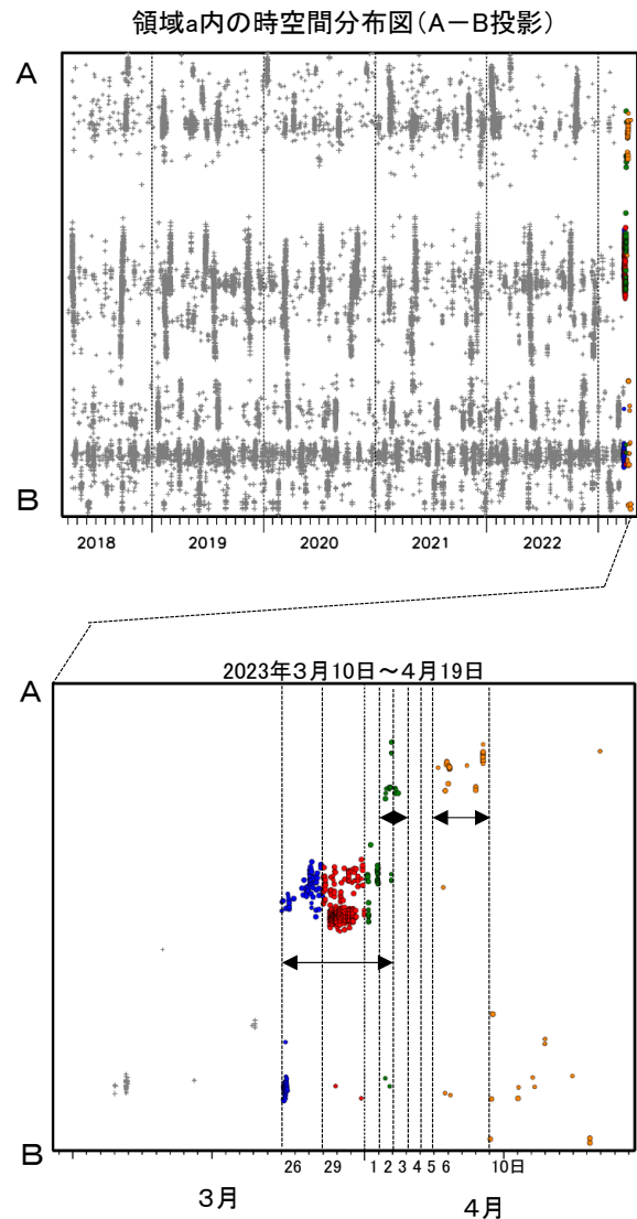
第 11 図 (a) 紀伊半島北部から東海の深部低周波地震活動とひずみ変化, 及び推定されるゆっくりすべり領域 Fig.11(a) Activity of deep low-frequency earthquakes in northern part of Kii Peninsula to Tokai region, and strain changes, and the estimated slow slip region.
