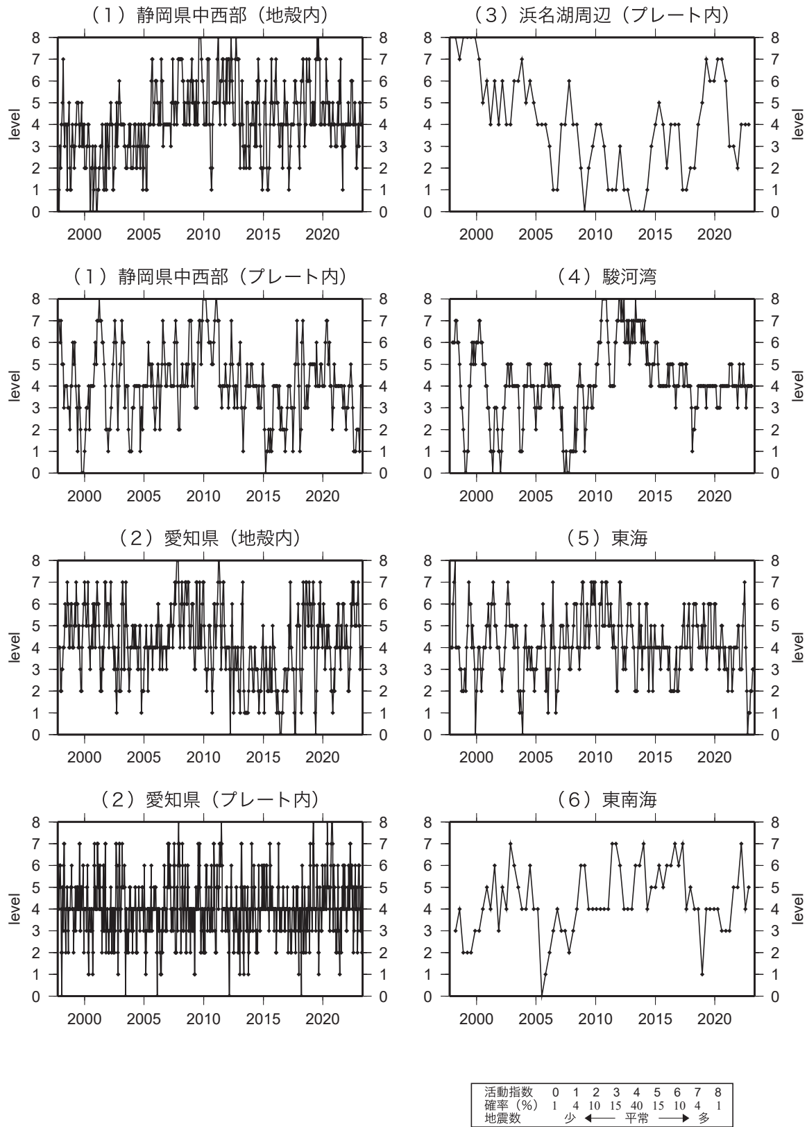
第 17 図 (a) 南海トラフ周辺の地震活動指数の推移 Fig.17(a) Time series of seismic activity levels in and around the Nankai Trough.
