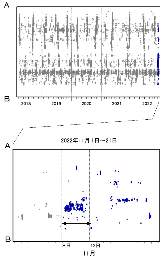
第 5 図 (a) 紀伊半島中部の深部低周波地震活動とひずみ変化, 及び推定されるゆっくりすべり領域 Fig.5(a) Activity of deep low-frequency earthquakes in central part of Kii Peninsula and strain changes, and the estimated slow slip region.
