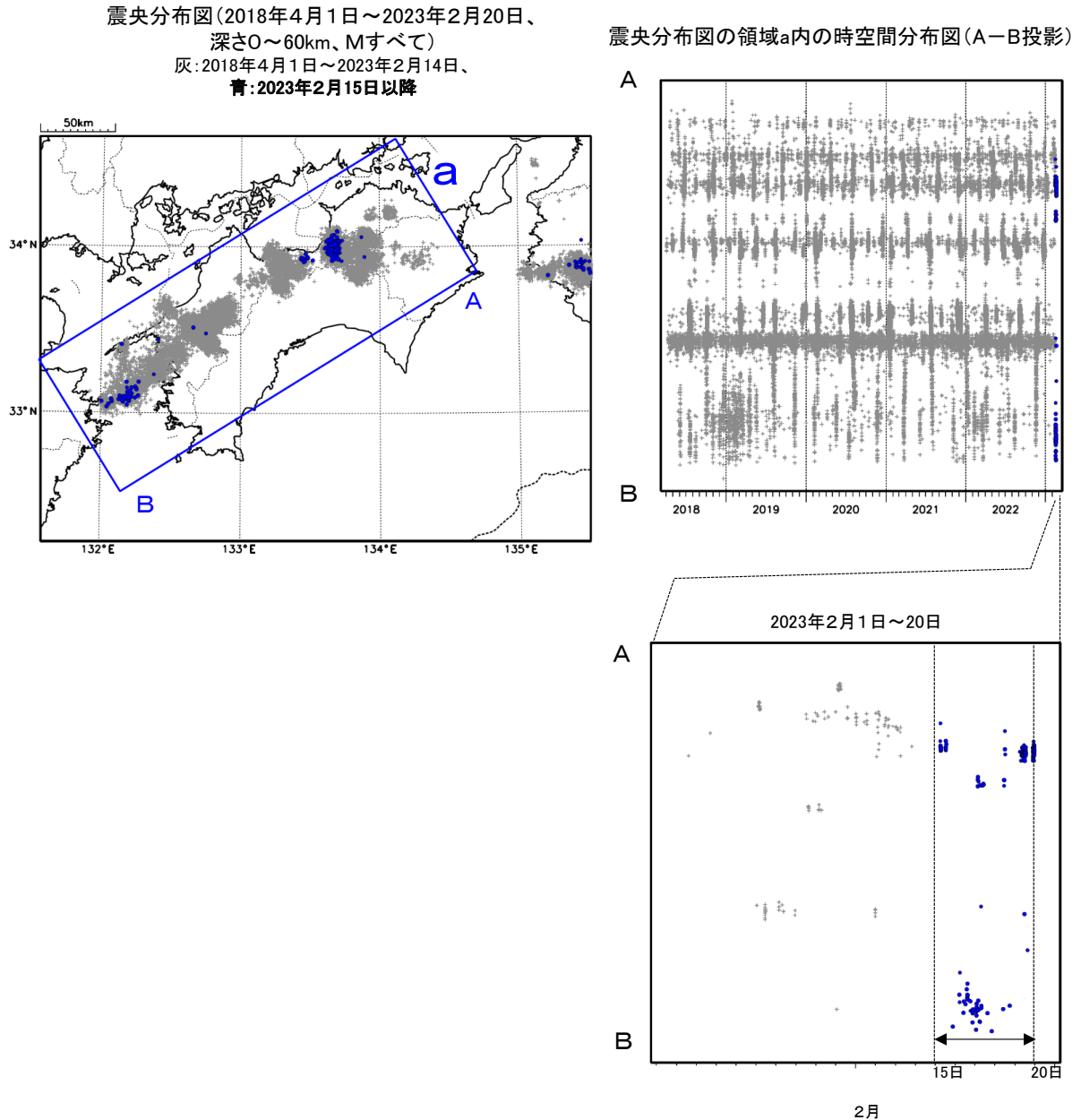
第 9 図 (a) 四国西部の深部低周波地震活動とひずみ変化, 及び推定されるゆっくりすべり領域 Fig.9(a) Activity of deep low-frequency earthquakes in western part of Shikoku region and strain changes, and the estimated slow slip region.
