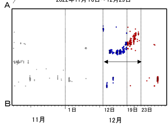
第 7 図 (a) 紀伊半島北部の深部低周波地震活動とひずみ変化，及び推定されるゆっくりすべり領域 Fig.7(a) Activity of deep low-frequency earthquakes in northern part of Kii Peninsula and strain changes, and the estimated slow slip region.
