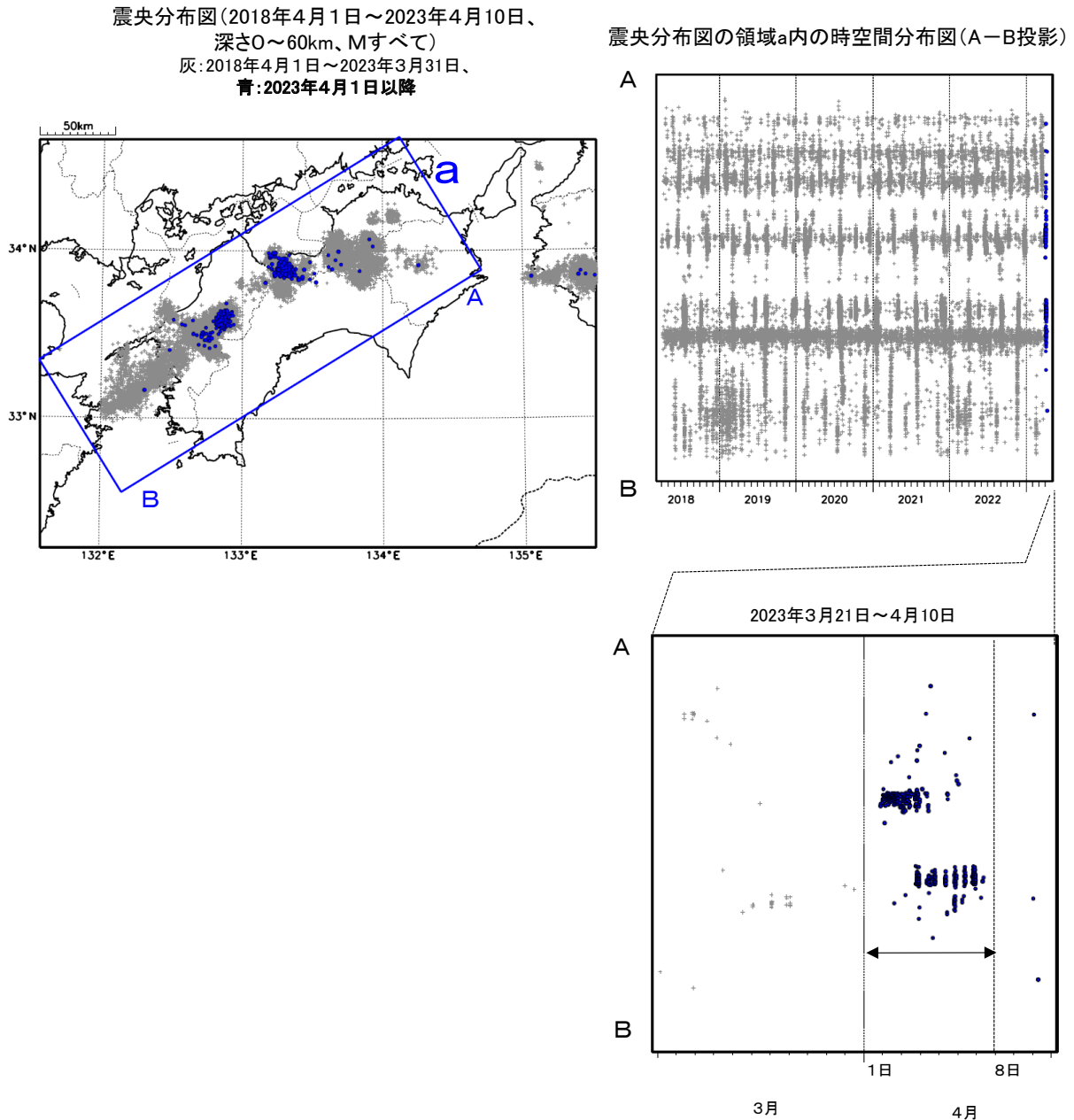
第 12 図 (a) 四国中部の深部低周波地震活動とひずみ・傾斜変化, 及び推定されるゆっくりすべり領域 Fig.12(a) Activity of deep low-frequency earthquakes in central part of Shikoku region and strain/tilt changes, and the estimated slow slip region.
