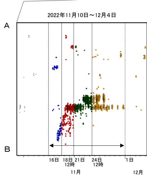
第 6 図 (a) 四国西部の深部低周波地震活動とひずみ変化, 及び推定されるゆっくりすべり領域 Fig.6(a) Activity of deep low-frequency earthquakes in western part of Shikoku region and strain changes, and the estimated slow slip region.
