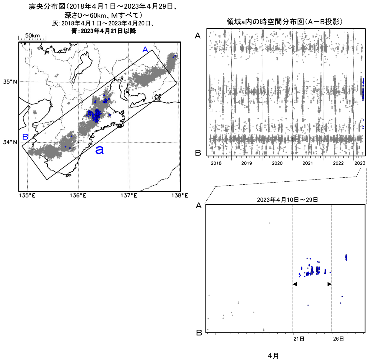
第 13 図 (a) 紀伊半島北部の深部低周波地震活動とひずみ・傾斜変化 Fig.13(a) Activity of deep low-frequency earthquakes in northern part of Kii Peninsula and strain/tilt changes.
