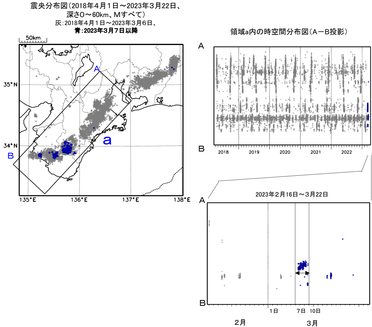
第 10 図 (a) 紀伊半島中部の深部低周波地震活動とひずみ変化, 及び推定されるゆっくりすべり領域 Fig.10(a) Activity of deep low-frequency earthquakes in central part of Kii Peninsula and strain changes, and the estimated slow slip region.
