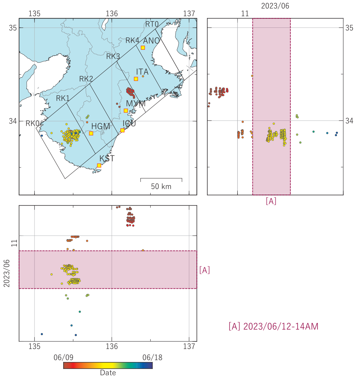
第 8 図 紀伊半島における低周波地震（気象庁一元化カタログによる）の時空間分布（2023/06/09 ～ 2023/06/17）. Fig. 8 Space-time distribution of low-frequency earthquakes by JMA unified hypocenter catalog in the Kii Peninsula from June 9 to 17, 2023.
