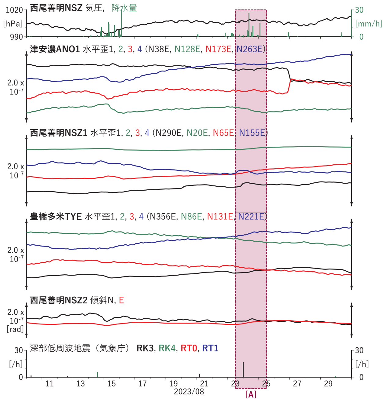
第 34 図 紀伊半島から東海地方における歪・傾斜の観測結果と低周波地震の検出数 (1) (2023/08/10 ~ 2023/08/30). Fig. 34 Observed strain and tilt data and detected number of low-frequency earthquakes in the Kii Peninsula and Tokai region from August 10 to 30, 2023 (1).
