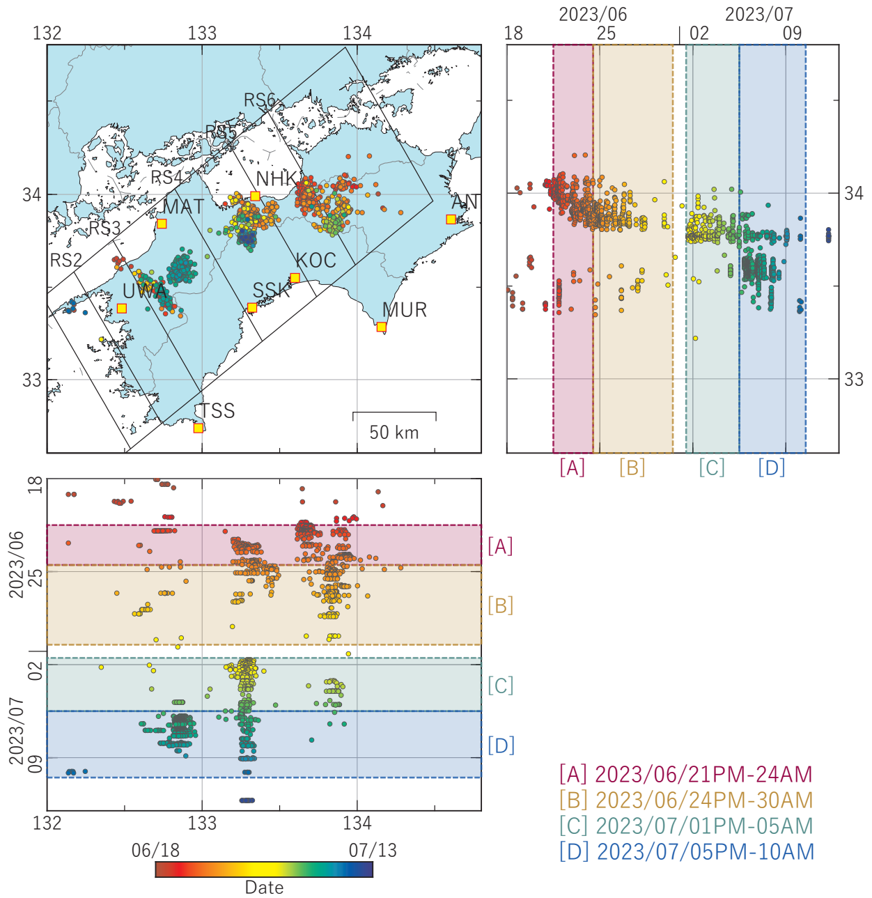
第 14 図 四国地域における低周波地震（気象庁一元化カタログによる）の時空間分布（2023/06/18 ~ 2023/07/12）. Fig. 14 Space-time distribution of low-frequency earthquakes by JMA unified hypocenter catalog in the Shikoku region from June 18 to July 12, 2023.
