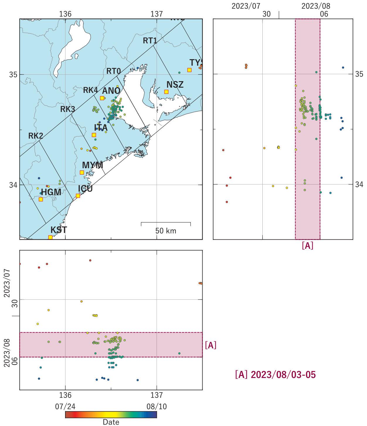
第 26 図 紀伊半島における低周波地震（気象庁一元化カタログによる）の時空間分布（2023/07/24 ～ 2023/08/09）. Fig. 26 Space-time distribution of low-frequency earthquakes by JMA unified hypocenter catalog in the Kii Peninsula from July 24 to August 9, 2023.
