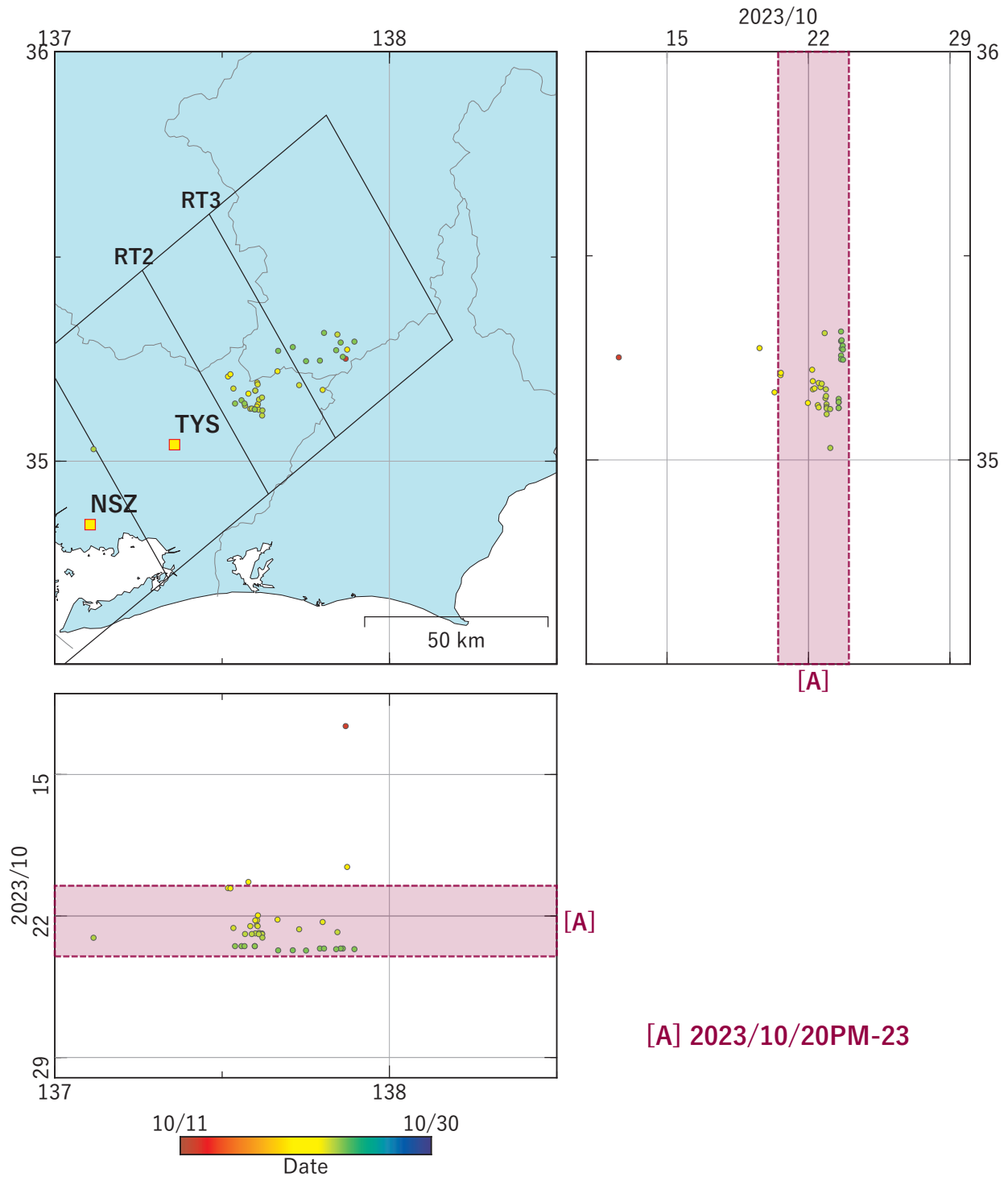
第 50 図 東海地方における低周波地震（気象庁一元化カタログによる）の時空間分布（2023/10/11 ~ 2023/10/29）. Fig. 50 Space-time distribution of low-frequency earthquakes by JMA unified hypocenter catalog in the Tokai region from October 11 to October 29, 2023.
