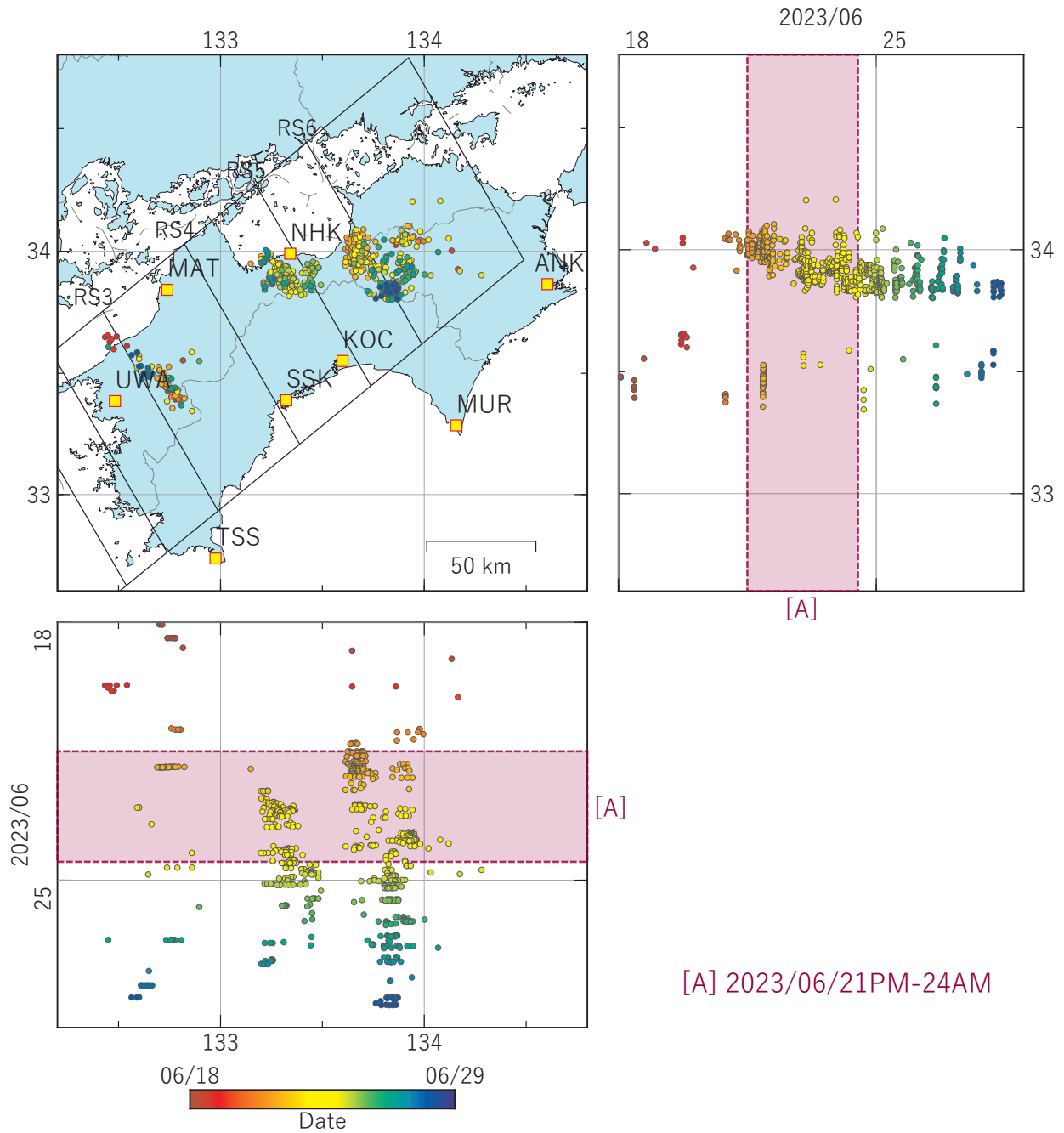
第 11 図 四国地方における低周波地震（気象庁一元化カタログによる）の時空間分布（2023/06/18～2023/06/28）. Fig. 11 Space-time distribution of low-frequency earthquakes by JMA unified hypocenter catalog in the Shikoku region from June 18 to 28, 2023.
