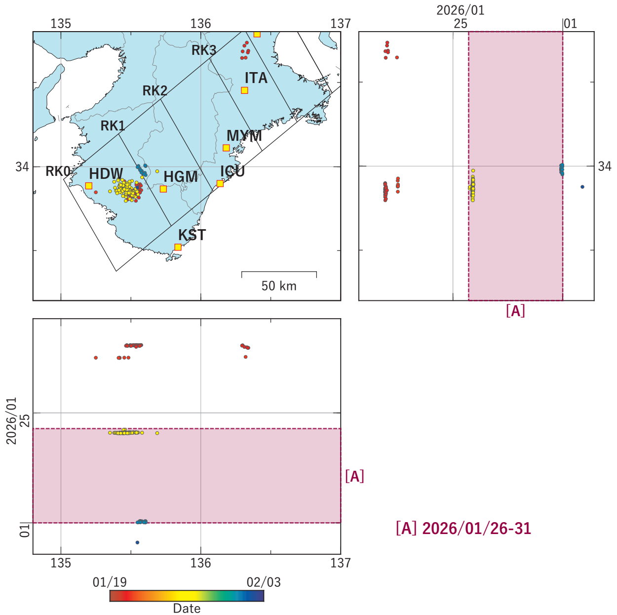
第 31 図 紀伊半島における低周波地震（気象庁一元化カタログによる）の時空間分布（2026/01/19–2026/02/02）. Fig. 31 Space-time distribution of low-frequency earthquakes by JMA unified hypocenter catalog in the Kii Peninsula from January 19 to February 02, 2026.
