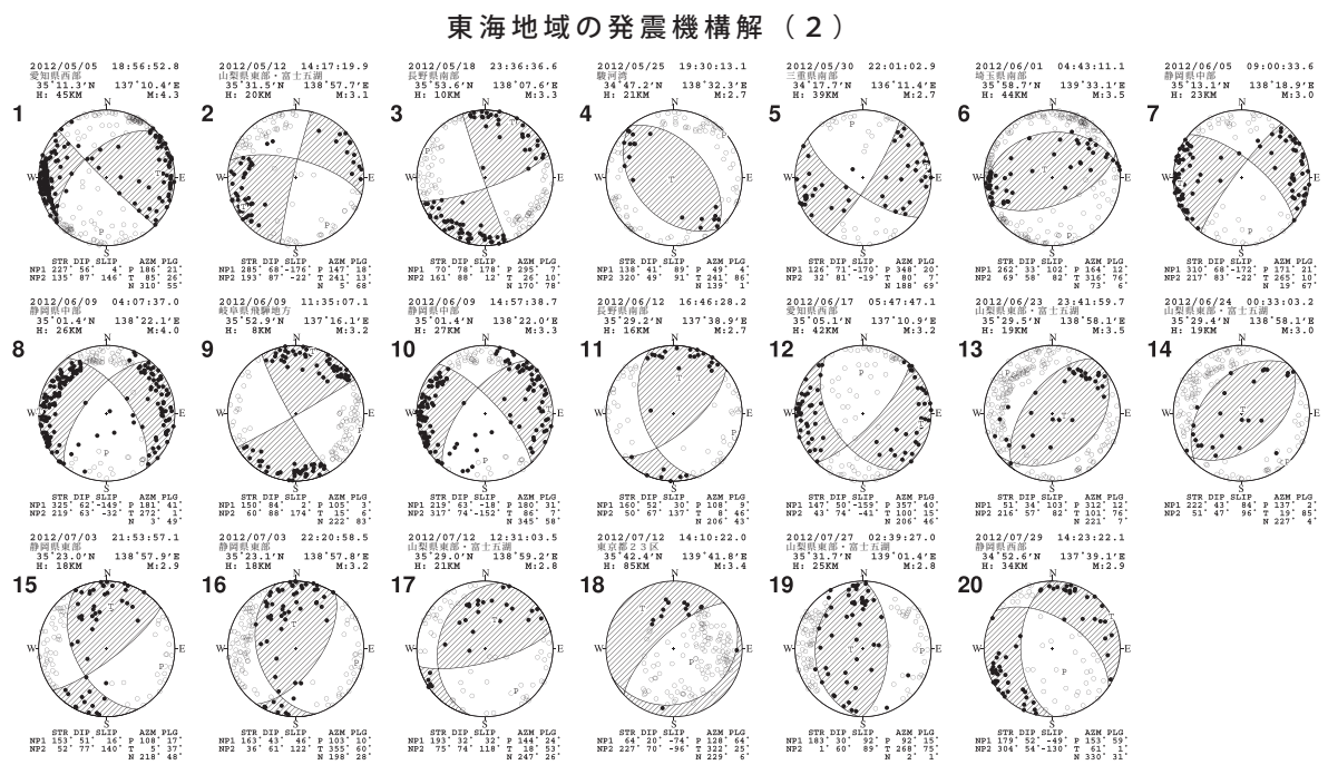
Fig.2 (a) Focal mechanism solutions for major earthquakes in the Tokai Districts (May – July 2012).
