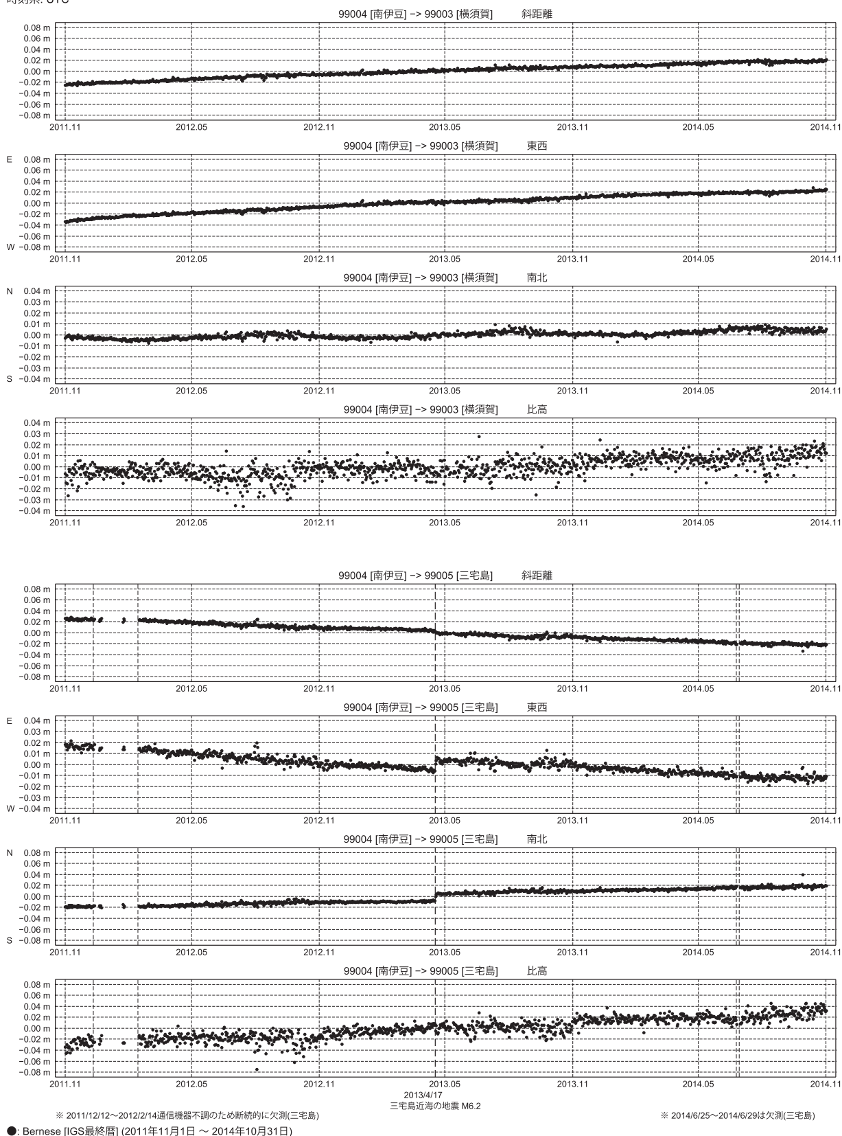
第3図 南伊豆基点での横須賀および三宅島のGPS連続観測結果 (2011/11/1 ~ 2014/10/31) Fig.3 Results of continuous GPS measurements for Yokosuka and Miyake-jima from November 1, 2011 to October 31, 2014.
