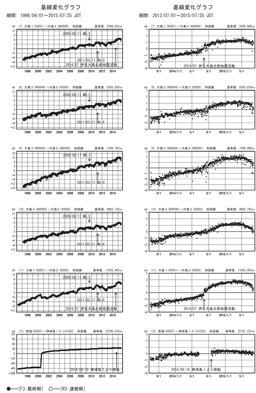
第8図 伊豆諸島北部GNSS連続観測結果 (斜距離) Fig. 8 Results of continuous GNSS measurements in the northern part of the Izu Islands (distance) (2/3).
