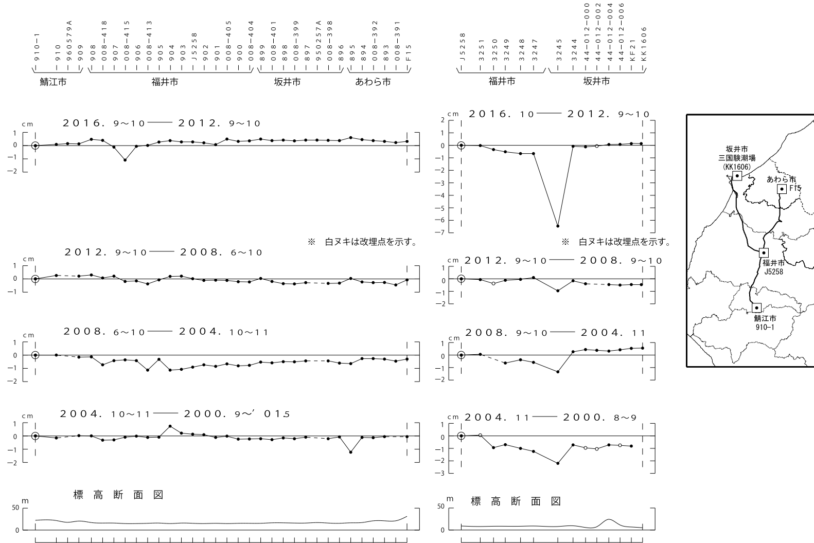
第1図 鯖江市～あわら市間、福井市～坂井市間の上下変動 Fig. 1 Results of leveling survey from Sabae city to Awara city, Fukui city to Sakai city.
