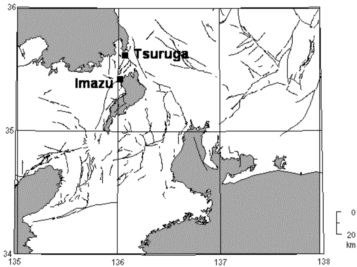
第1図 今津・敦賀観測点の位置. 図中の線は活断層研究会(1991)による活断層の位置. Fig. 1 Locational map of crustal deformation observation stations (Imazu and Tsuruga). The lines in the figure are the position of active faults by The Research Group for Active Faults of Japan (1991).
