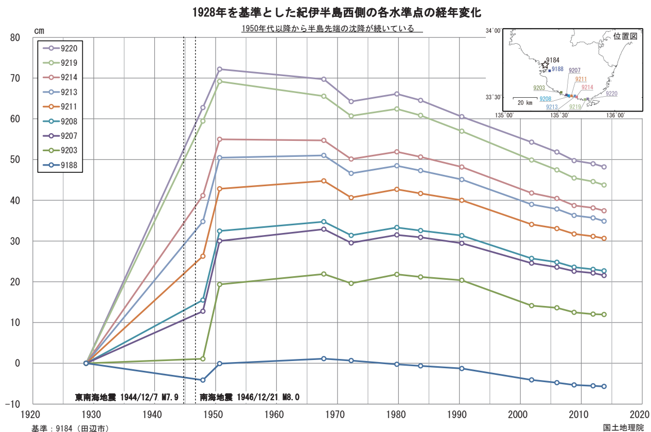
第4図 紀伊半島西側の水準点の上下変動経年変化 (1928年度基準・J9184 固定) Fig. 4 Time series of vertical movement from 1928 on the benchmarks along the leveling route in western Kii Peninsula referred to J9184.
