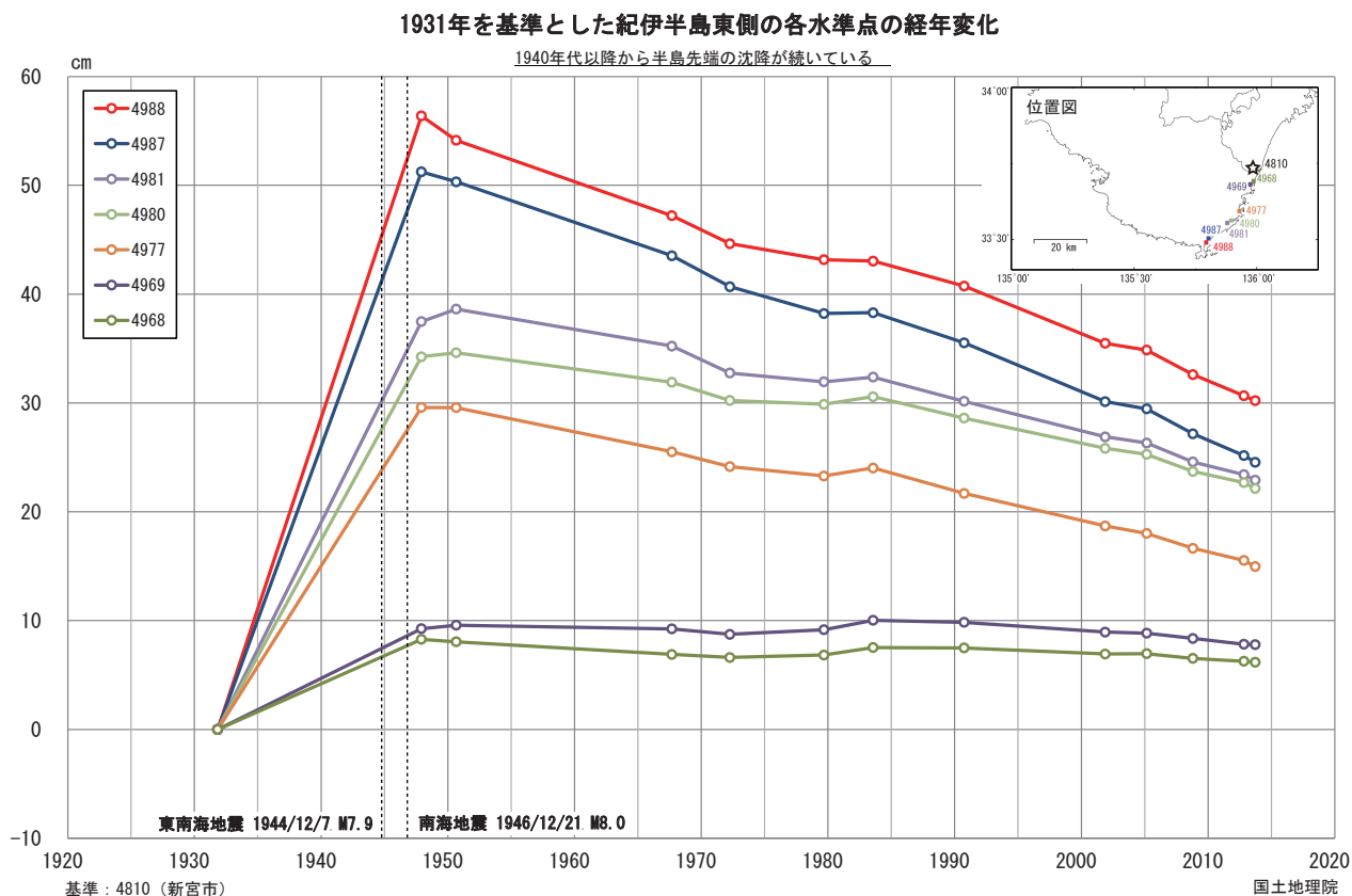
第5図 紀伊半島東側の水準点の上下変動経年変化 (1931年度基準・J4810 固定) Fig. 5 Time series of vertical movement from 1931 on the benchmarks along the leveling route in eastern Kii Peninsula referred to J4810.
